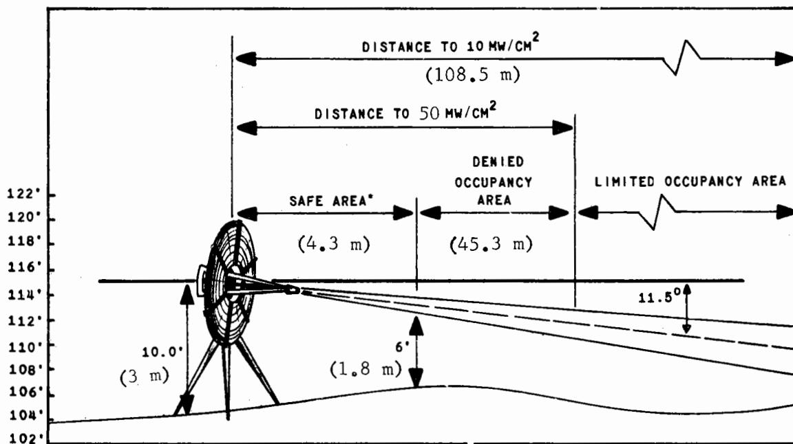
ELEVATION VIEW
