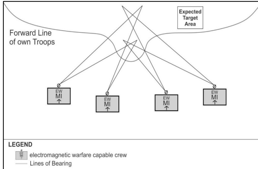
Figure 6-4. Concave baseline
