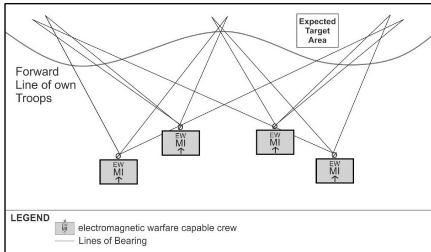
Figure 6-5. Convex baseline
