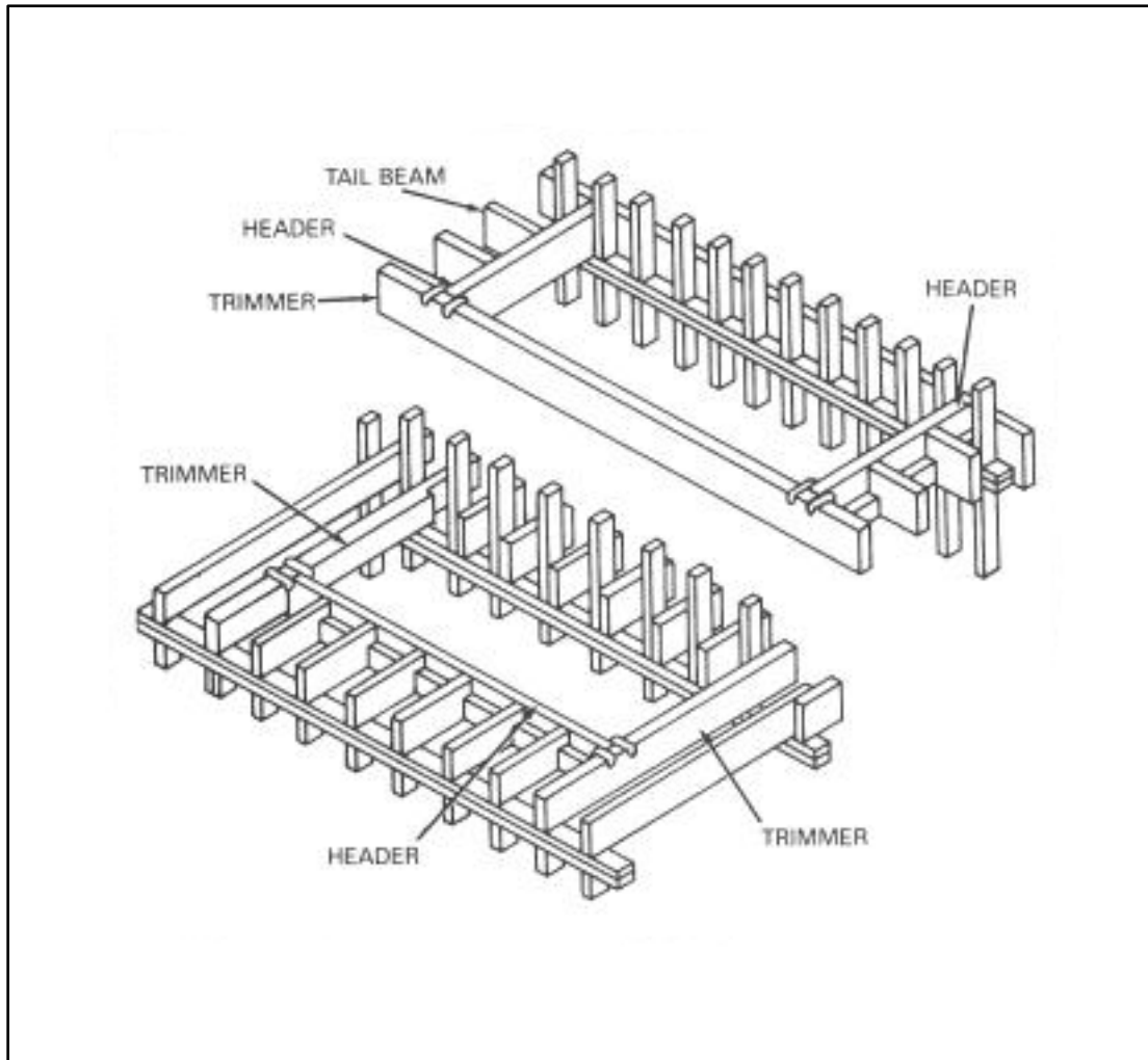
Figure 6-23. Floor openings
