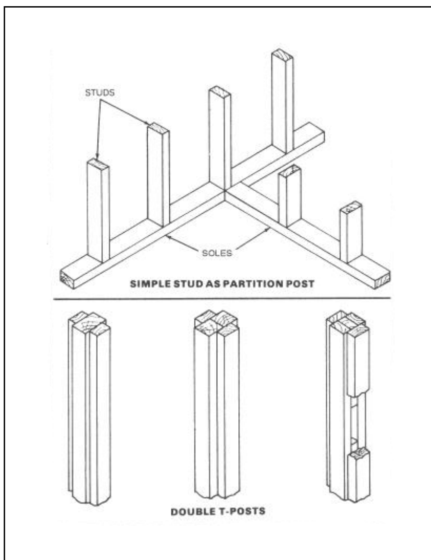
Figure 6-34. Partition posts
