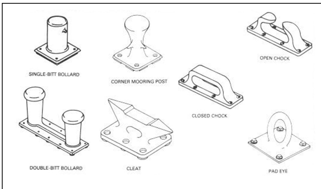
Figure 11-14. Mooring hardware
