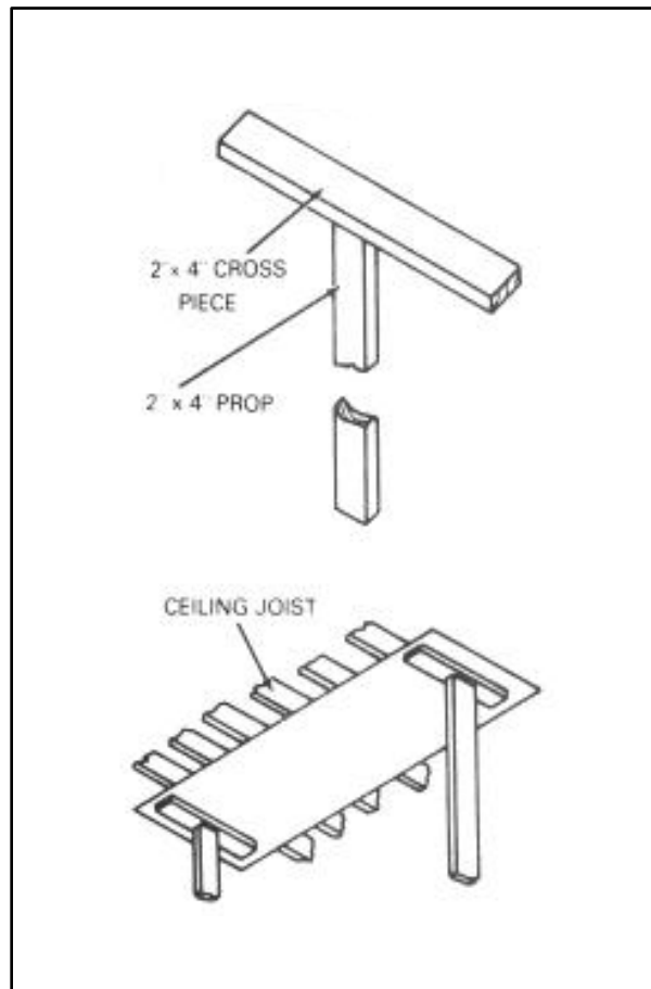
Figure 9-10. Brace for holding ceiling panels
