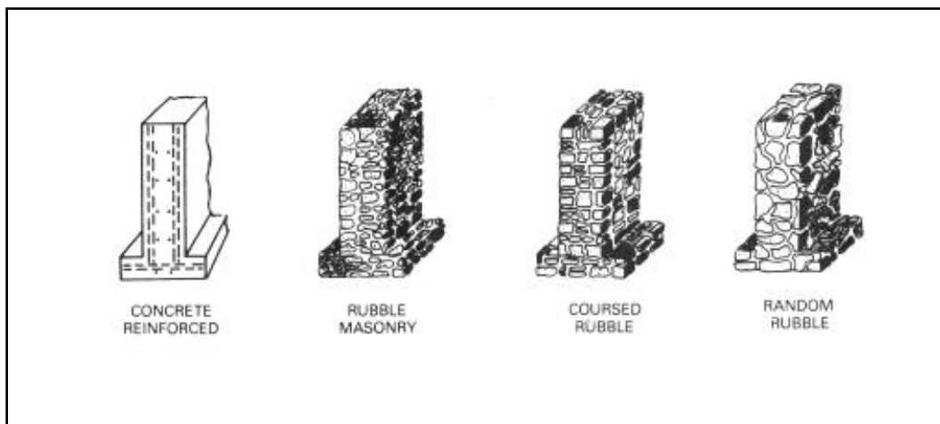
Figure 4-5. Foundation walls
