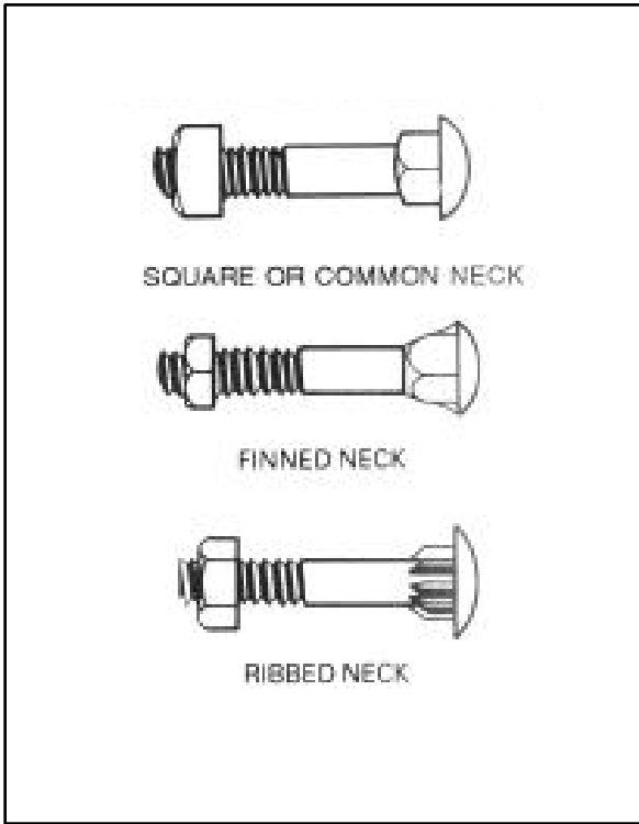
Figure 2-11. Carriage bolts
