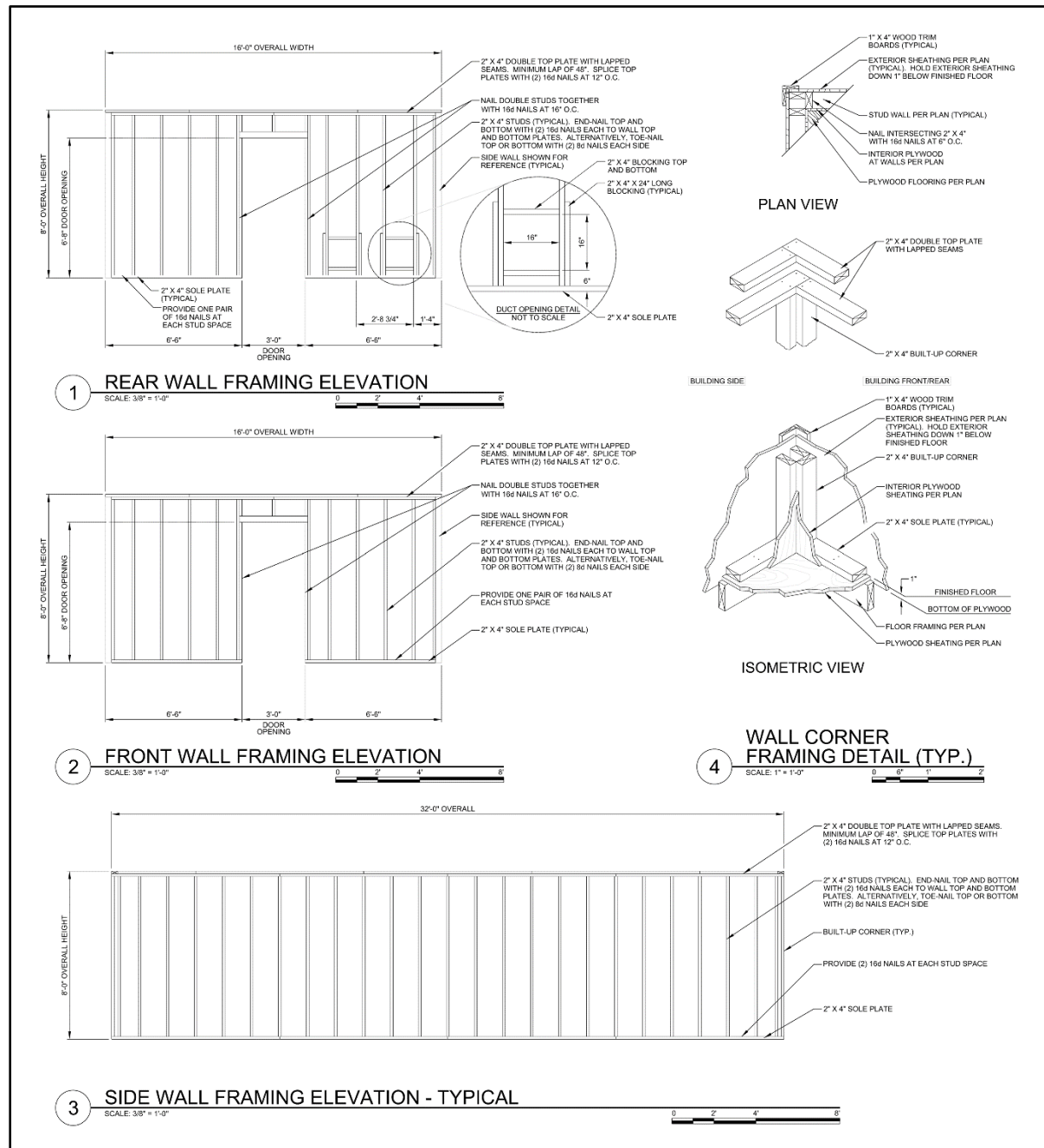
Figure 1-17. Typical wall-panel framing details (continued)
