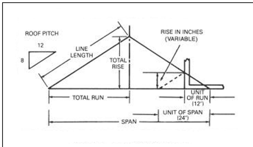
Figure 7-6. Determining roof pitch
