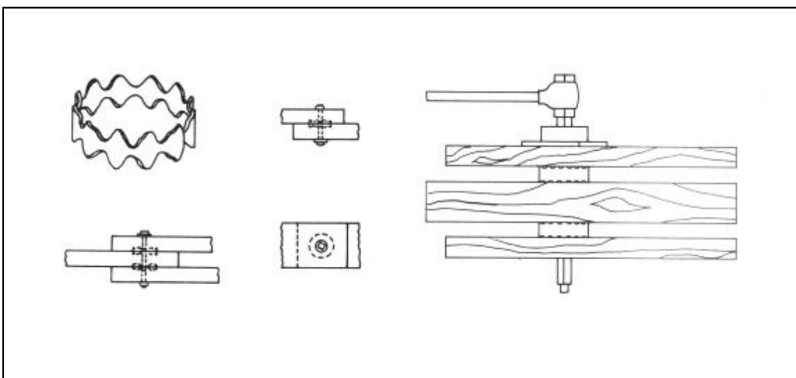
Figure 2-19. Toothed-ring installation
