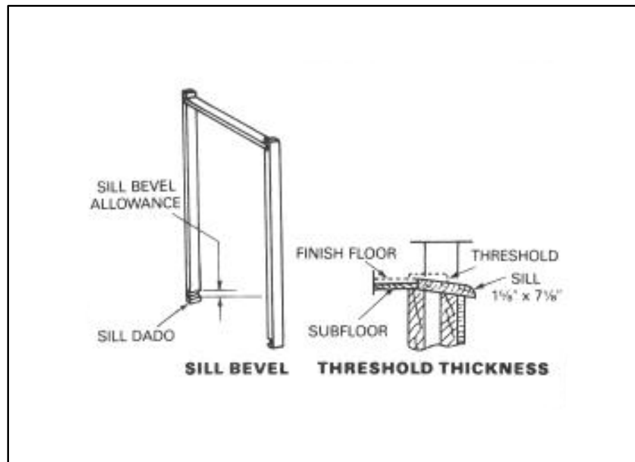
Figure 8-8. Jamb allowances
