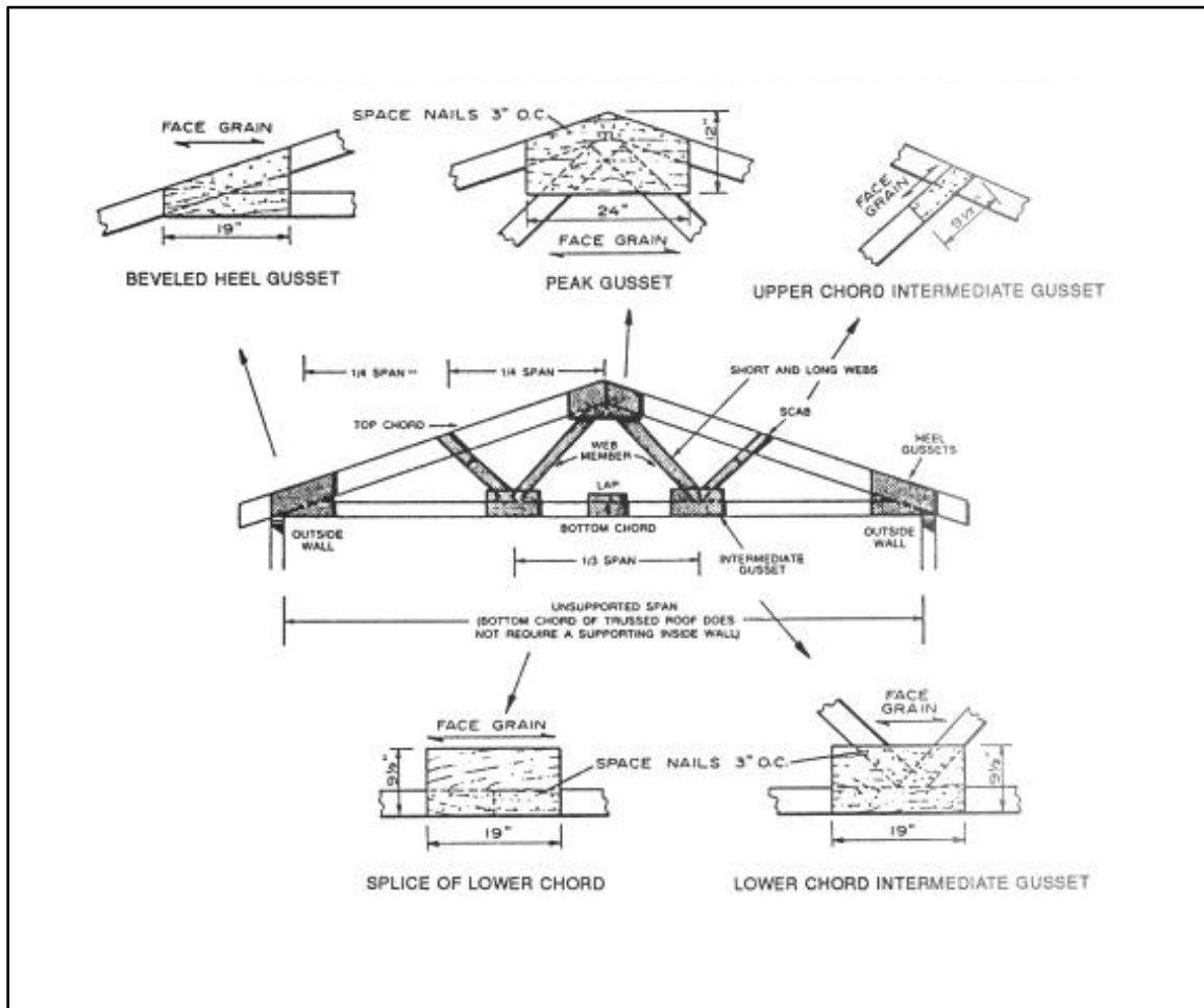
Figure 1-20. W-truss
