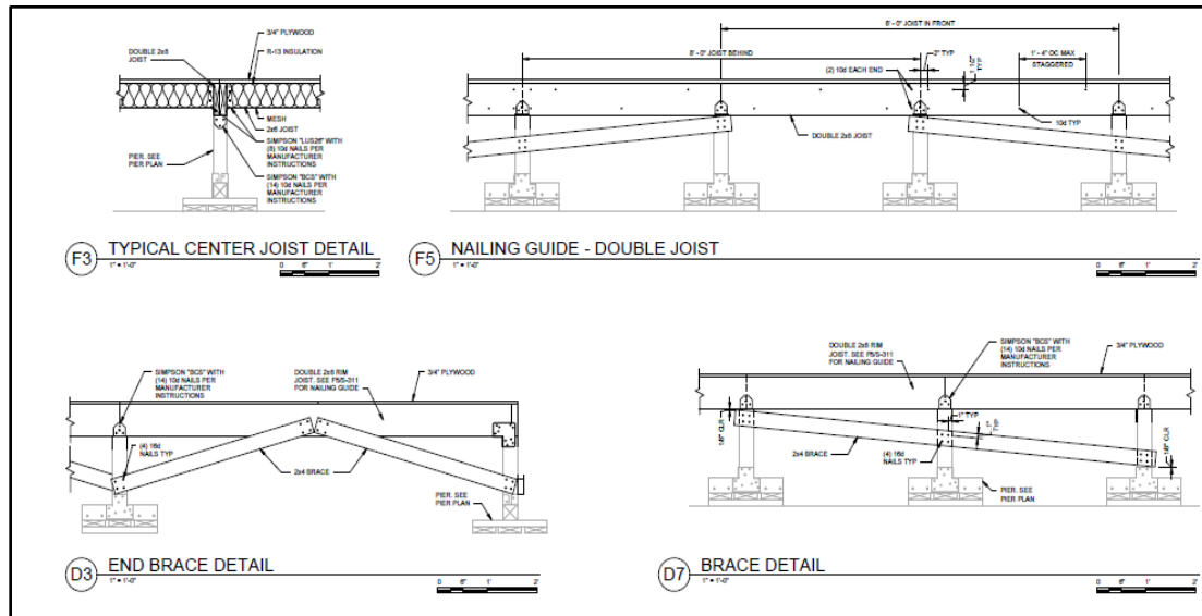
Figure 1-9. Typical floor plan section details
