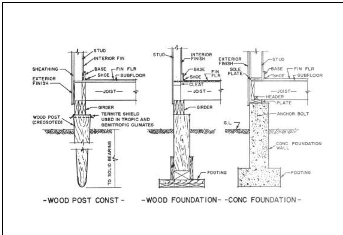
Figure 1-14. Typical foundation wall, post, footing, and girder details
