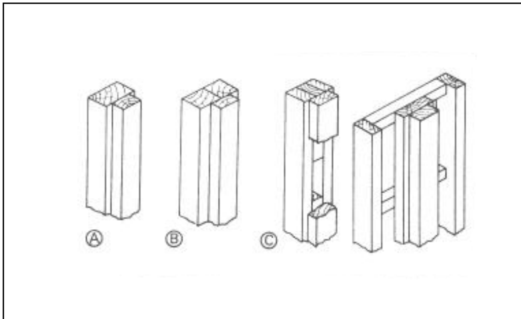
Figure 6-33. T-Post construction
