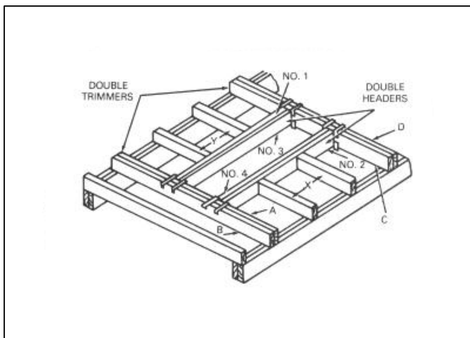
Figure 6-25. Floor-opening construction
