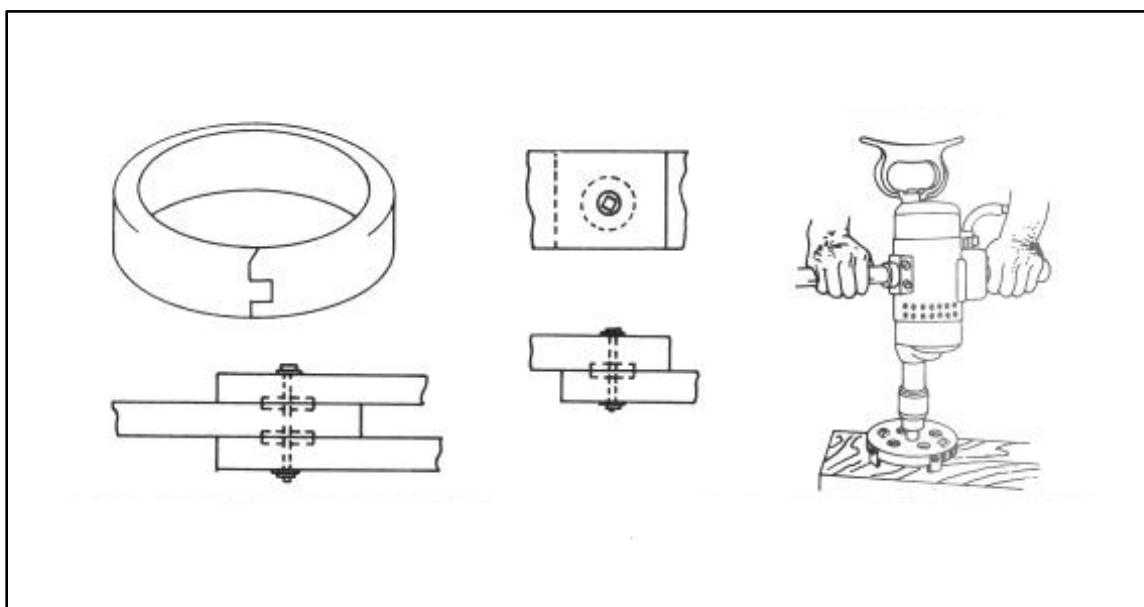
Figure 2-18. Split-ring installation
