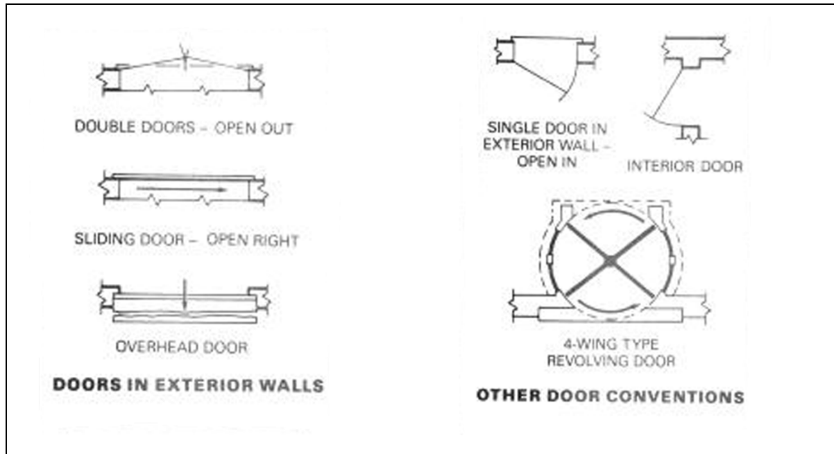
Figure 1-2. Door symbols
