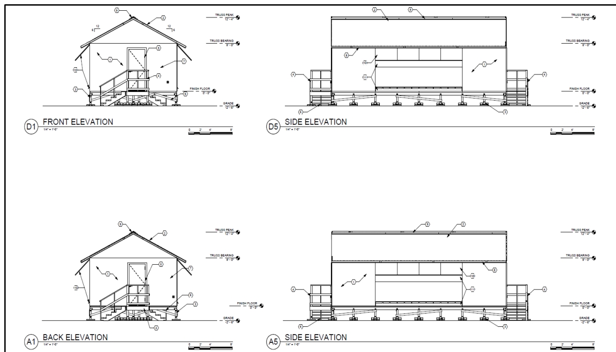
Figure 1-6. Elevation drawing
