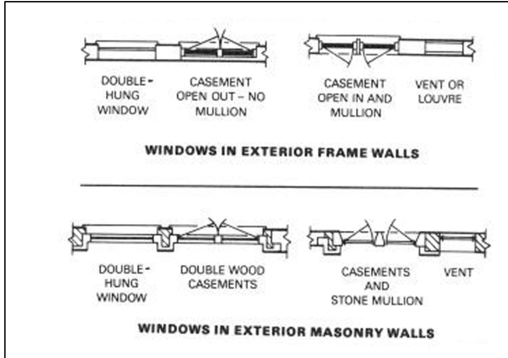
Figure 1-1. Window symbols
