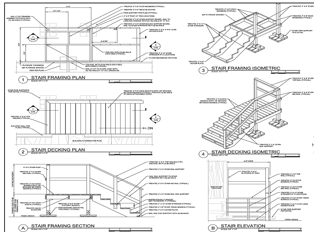
Figure 1-13. Stairway and steps
