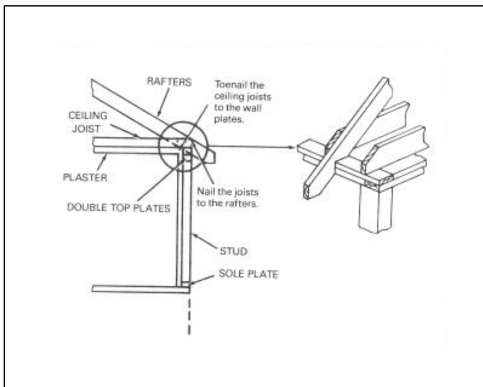
Figure 6-45. Built-up plate supporting joist and roof rafters
