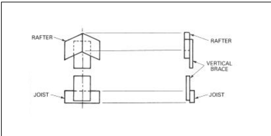
Figure 7-16. Truss assembly
