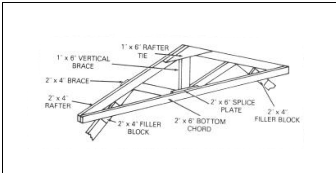
Figure 7-17. Assembling a typical truss
