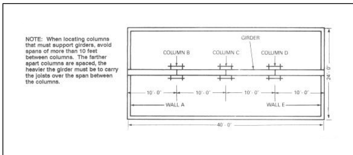
Figure 6-16. Column spacing
