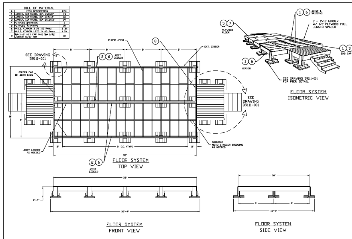
Figure 1-16. Floor framing details (20-foot-wide building)
