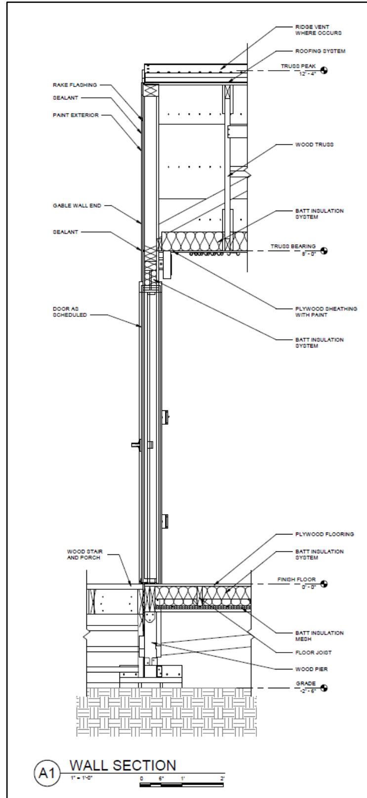
Figure 1-11. Typical wall section
