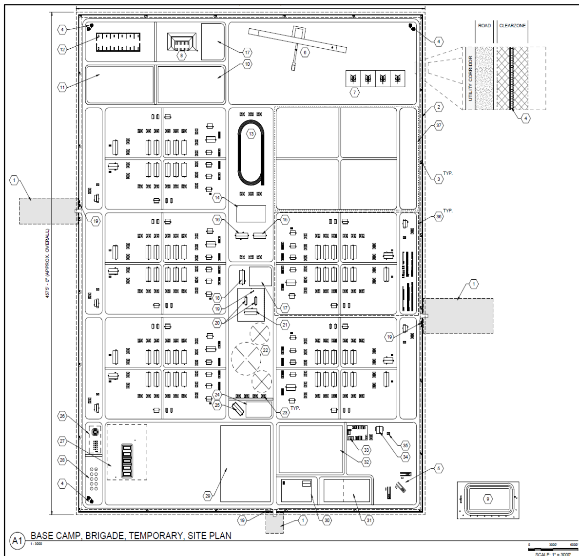
Figure 1-5. Base camp, temporary, site plan
