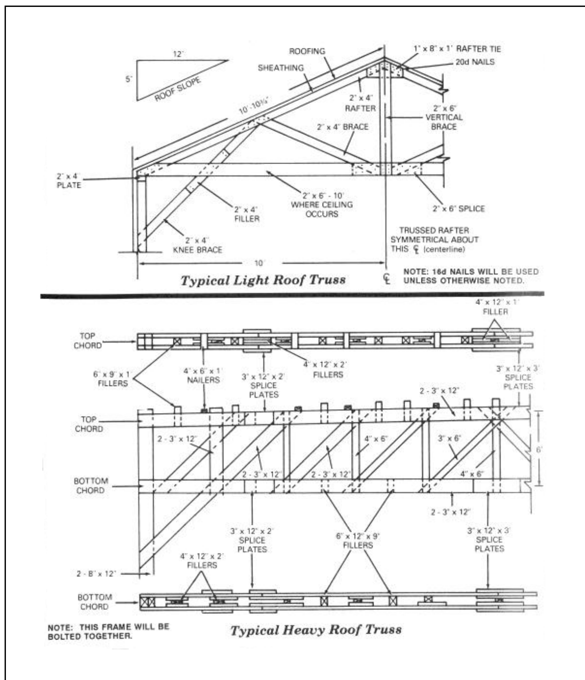
Figure 1-21. Roof trusses
