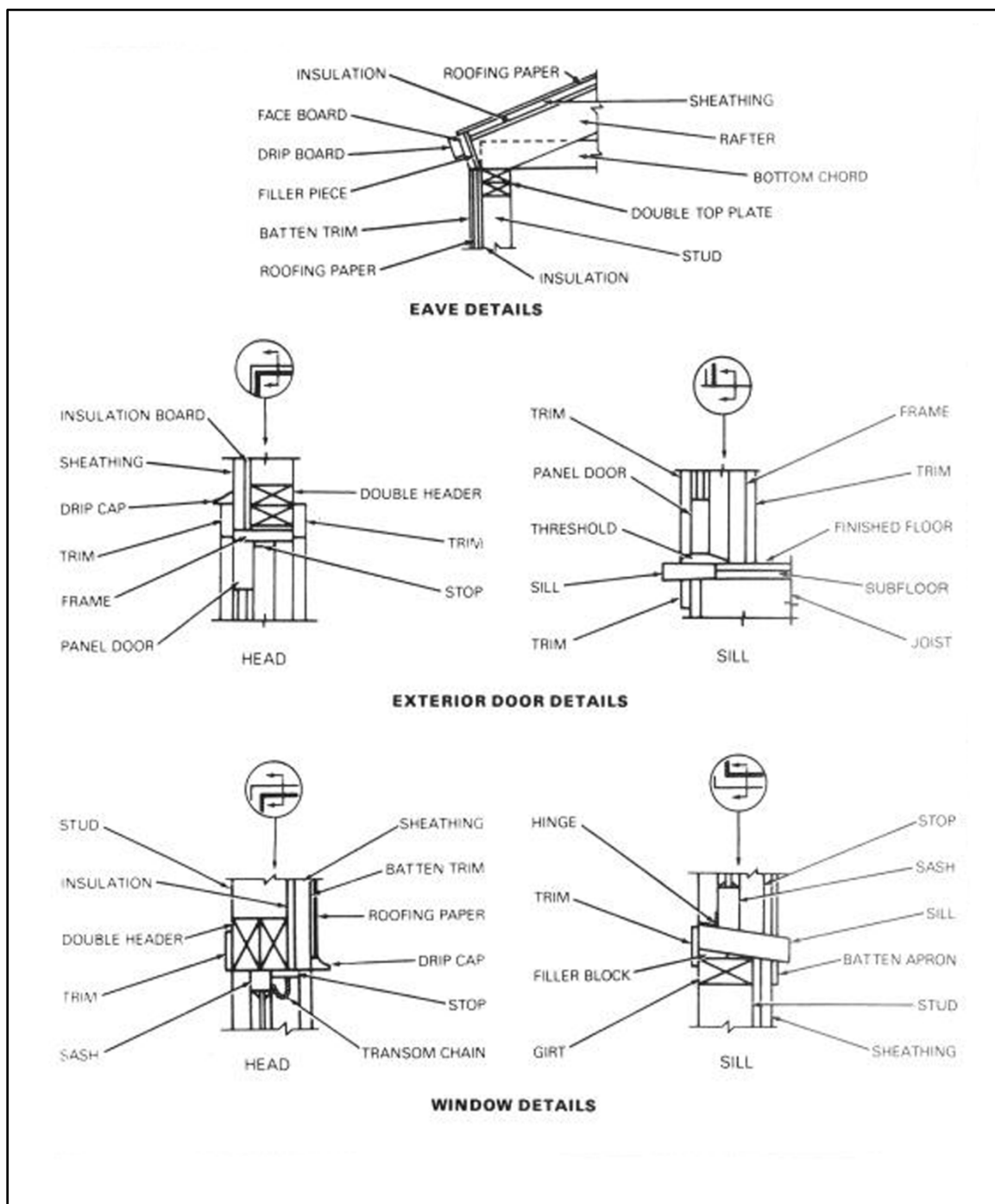
Figure 1-12. Typical eave, door, and window details
