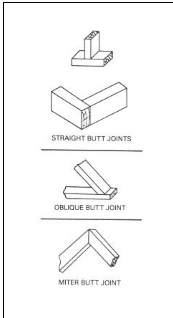
Figure 6-4. Butt joints
