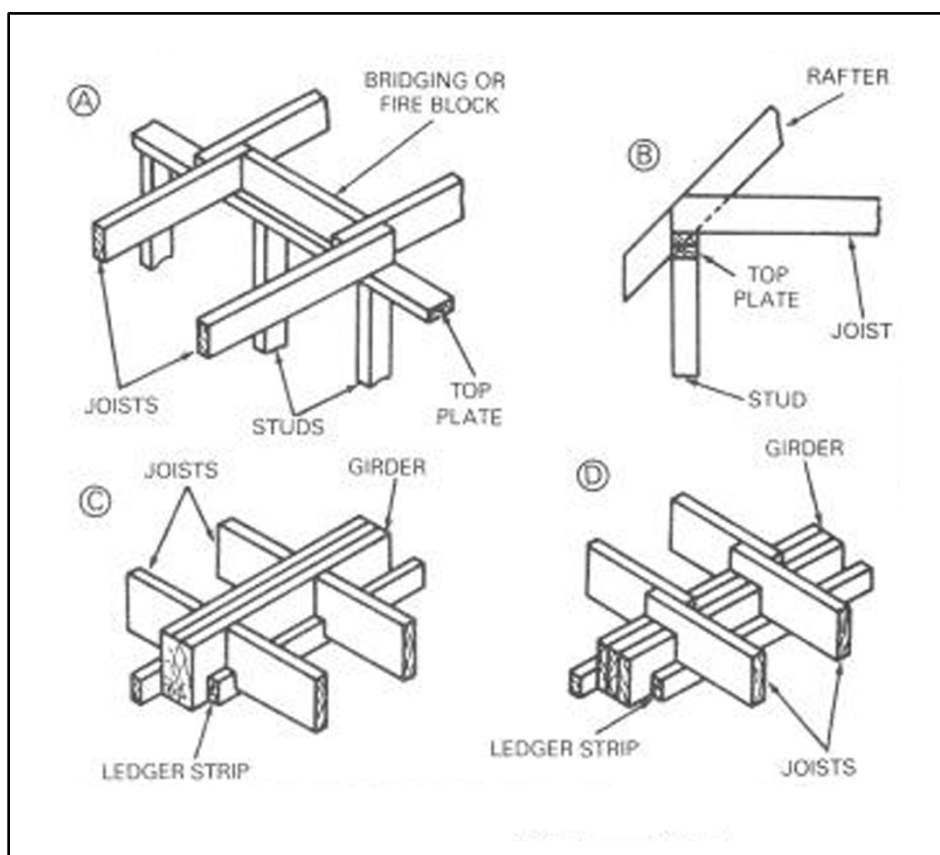
Figure 6-21. Top plates and ledgers
