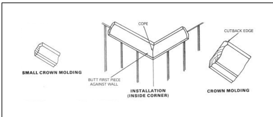
Figure 9-12. Ceiling molding
