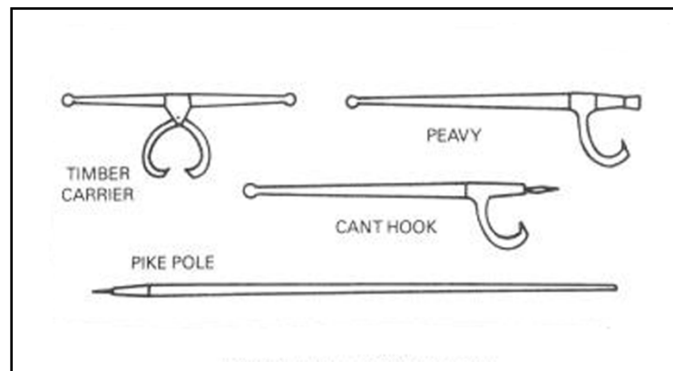
Figure 11-2. Logger's tools
