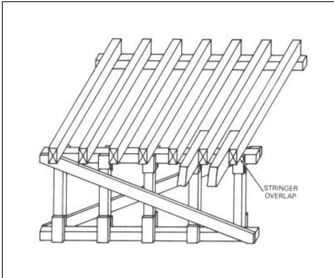
Figure 10-13. Stringer placement
