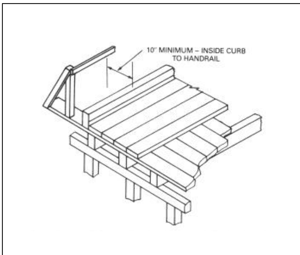
Figure 10-17. Solid-plank deck
