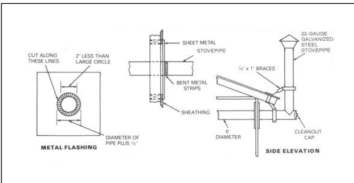
Figure 6-48. Installing stovepipe
