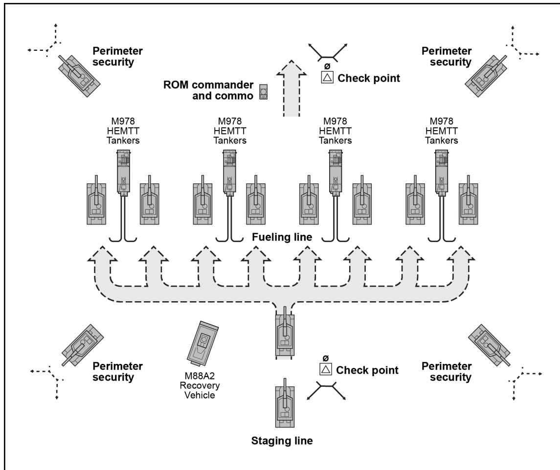
Figure G-6. ROM alternate configuration layout
