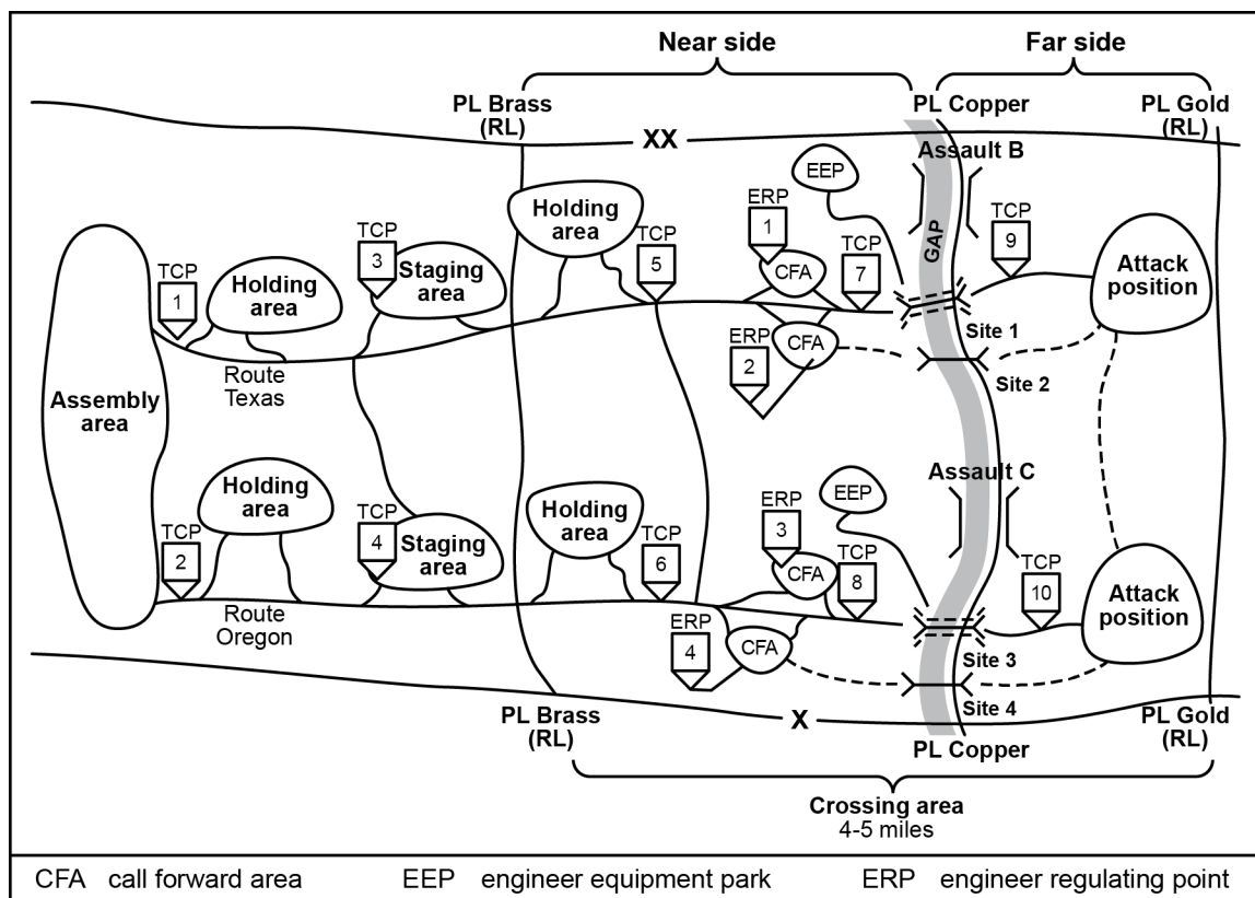
Figure A-2. Example gap crossing graphic control measures
