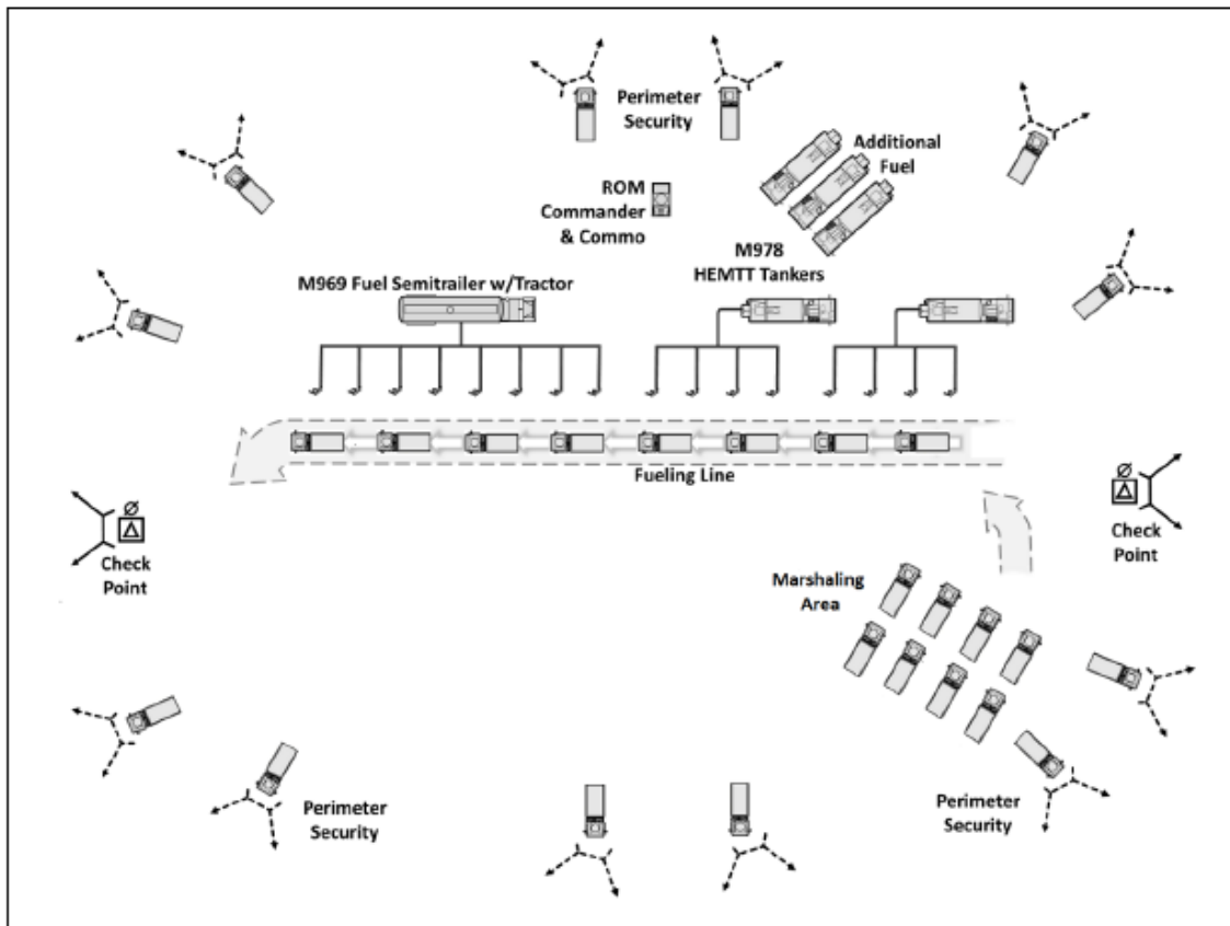
Figure G-5. Example refuel on the move layout
