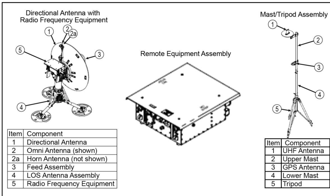
Figure C-10. Remote equipment assembly
