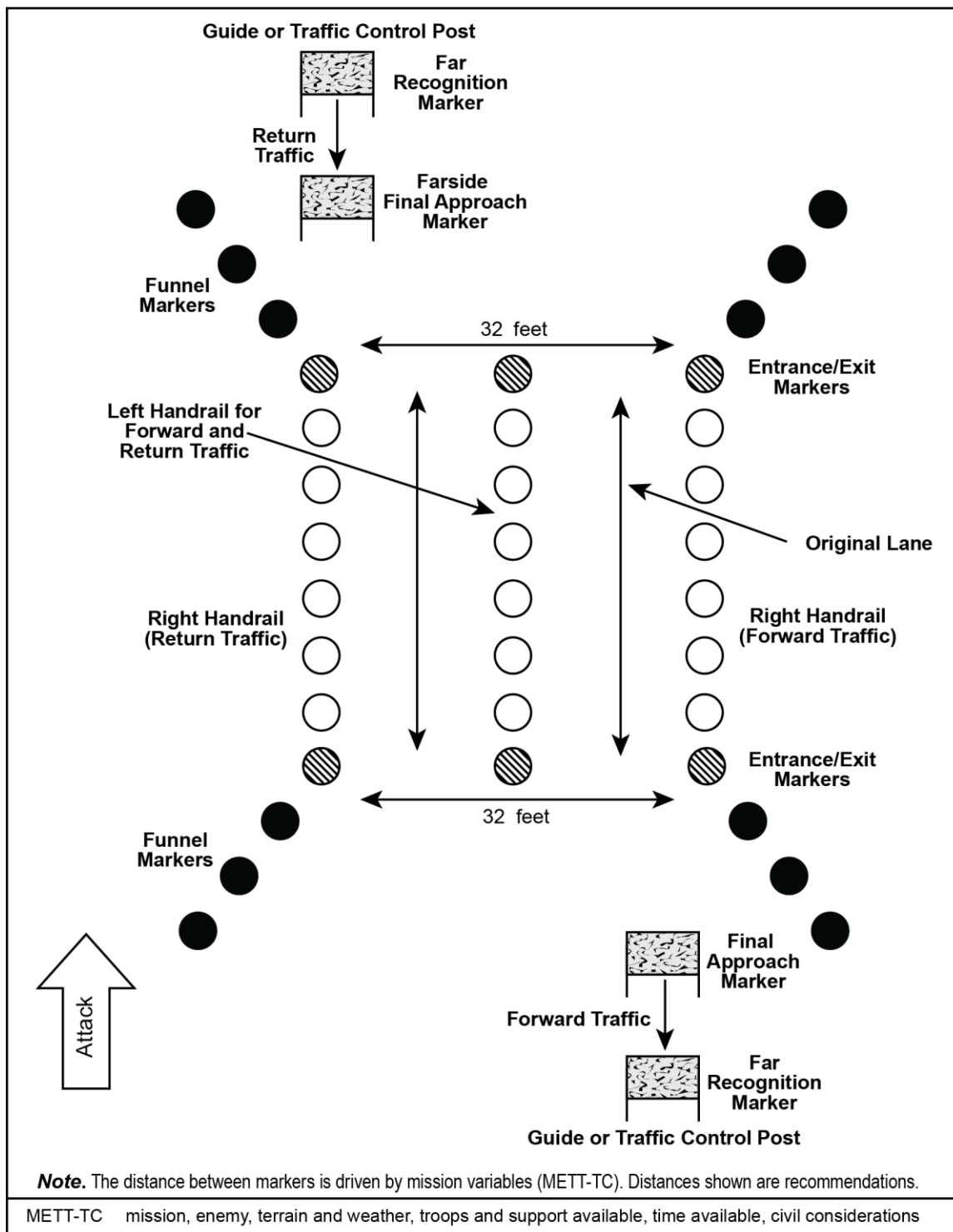
Figure F-3. Full lane-marking pattern
