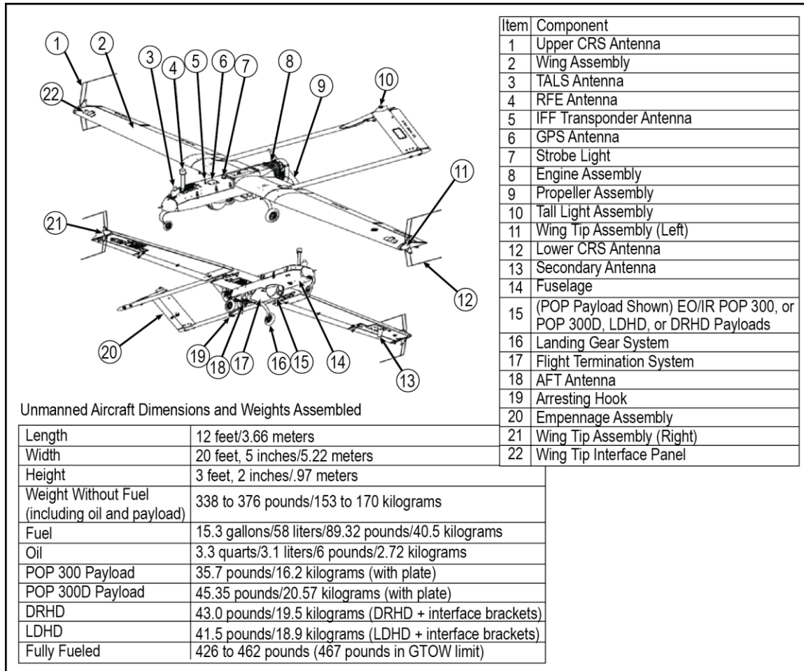
Figure C-6. Unmanned aircraft components
