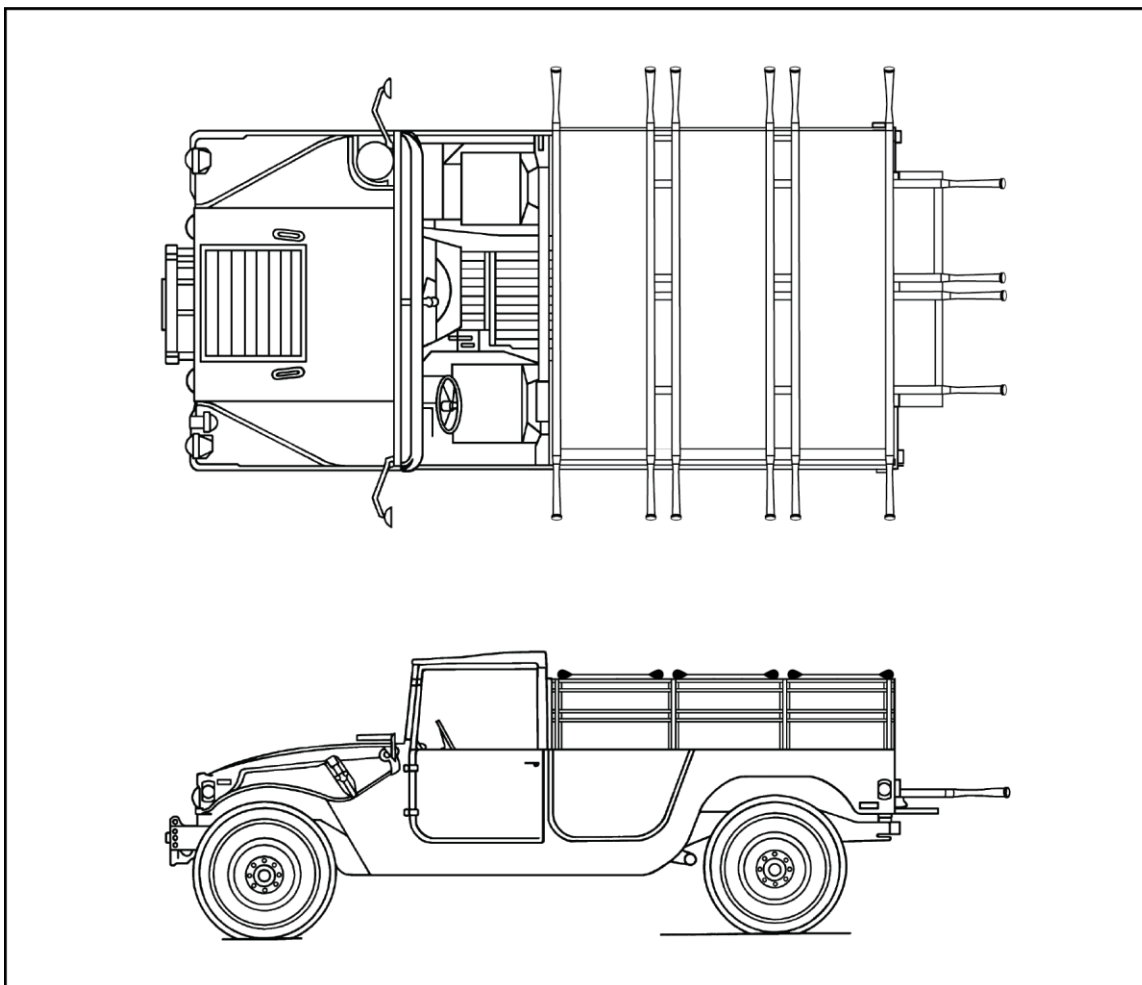
Figure J-17. M998 truck, cargo/troop carrier, HMMWV (two-man configuration)
