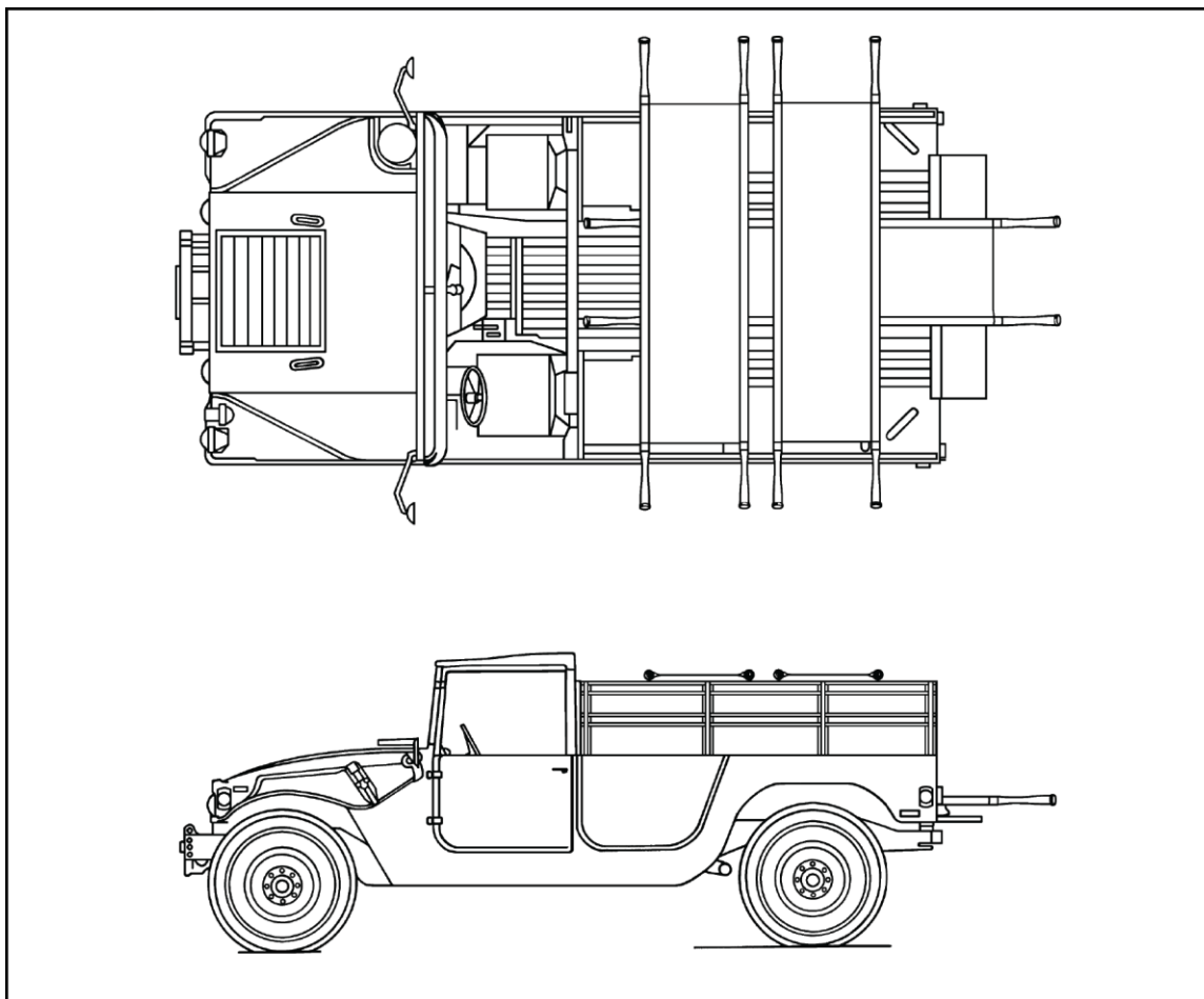
Figure J-16. M998 truck, cargo/troop carrier, HMMWV (four-man configuration)
