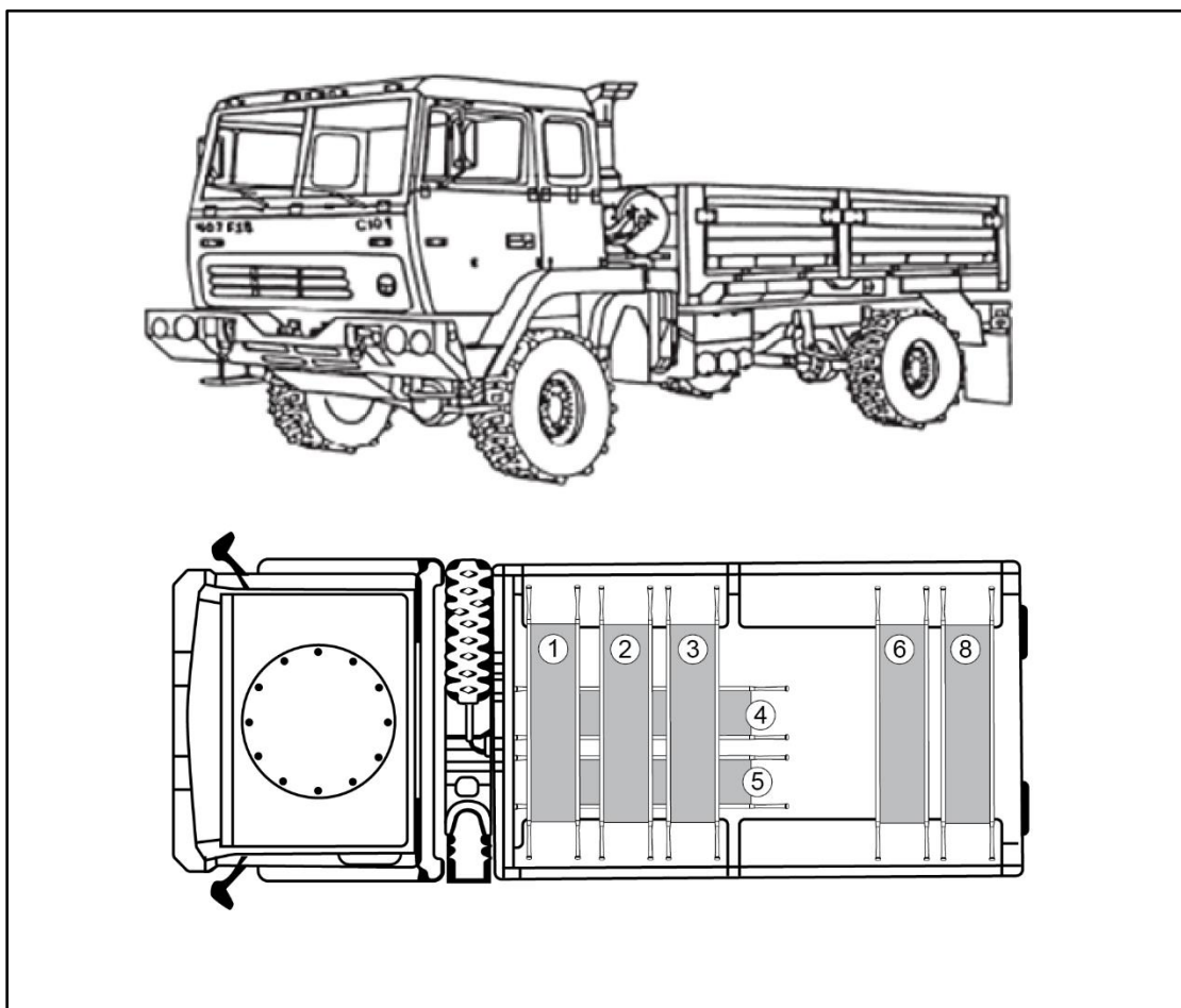
Figure J-19. Loading the M1081, light medium tactical vehicle
