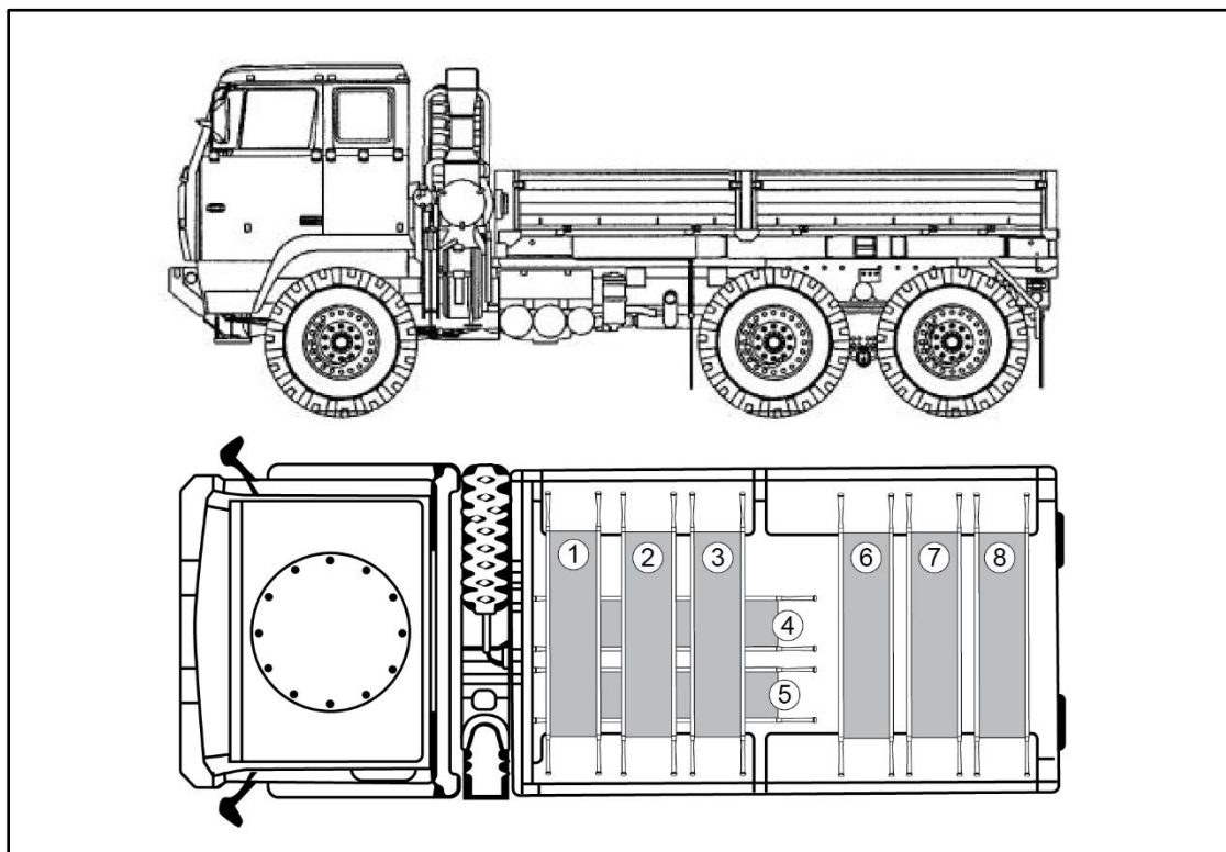
Figure J-18. Loading the M1093, medium tactical vehicle
