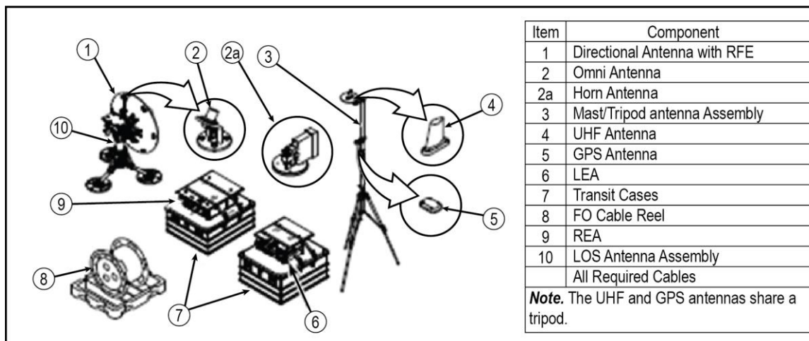
Figure C-8. Ground data terminal
