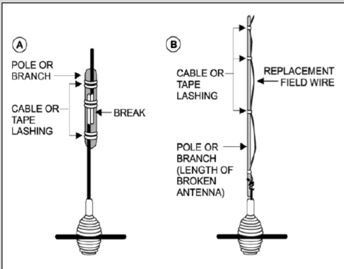
Figure N-2. Whip antenna body repair
