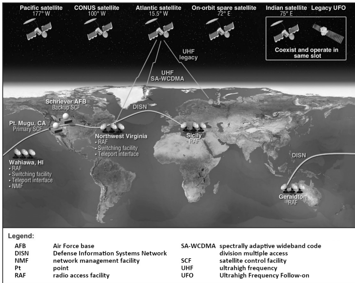
Figure B-4. Wideband code division multiple access network architecture
