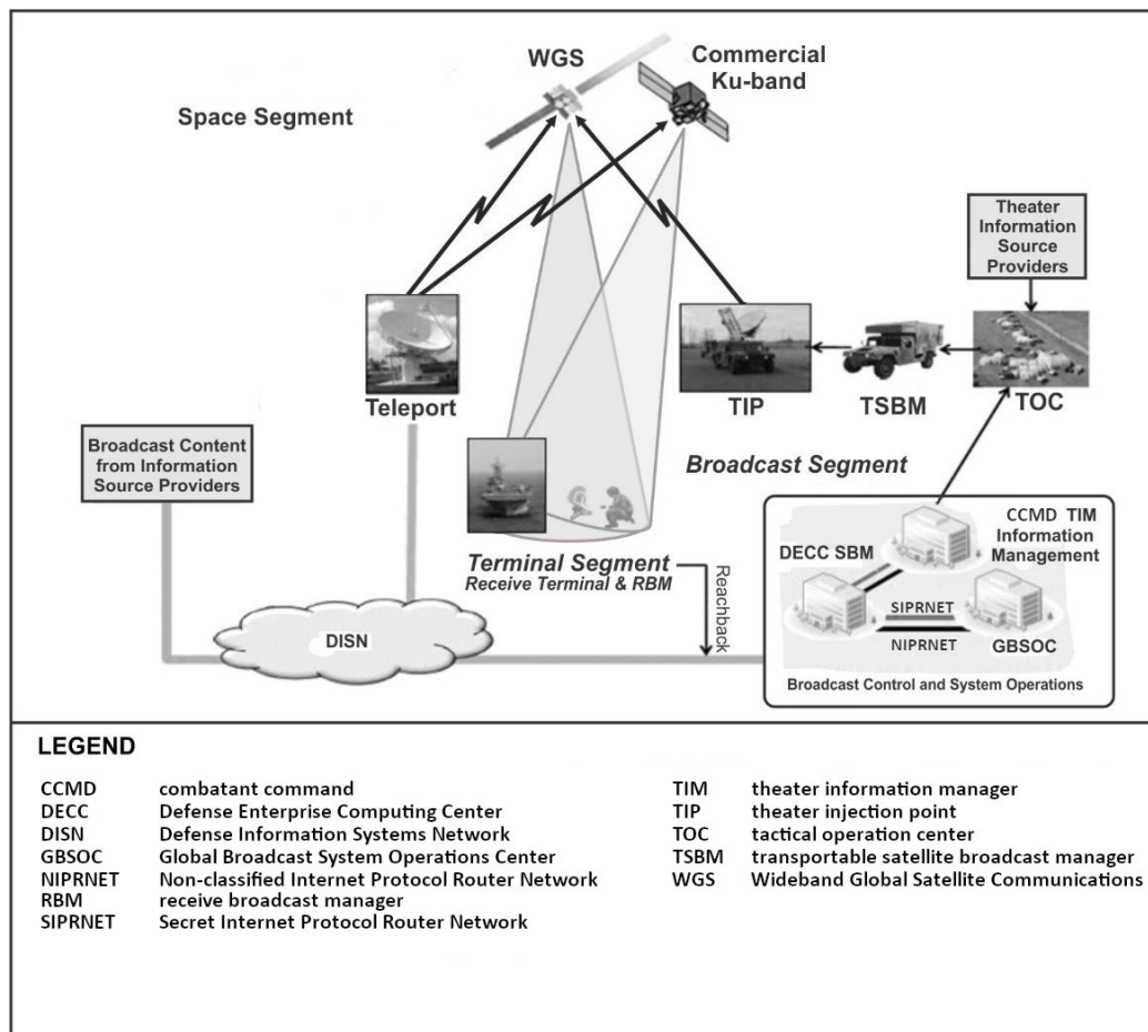
Figure C-1. Global Broadcast System broadcast and space segments
